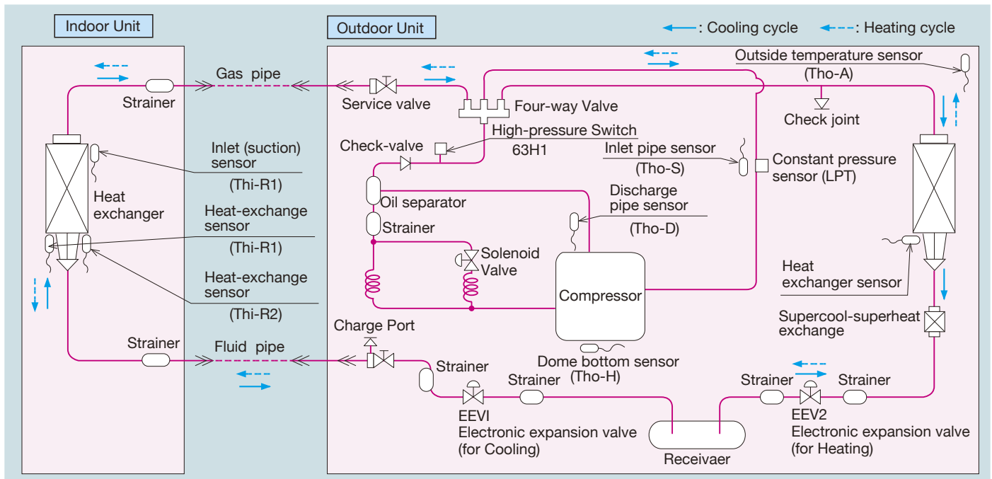
Fig. 7 Receiver circuit The receiver is located far from the compressor, where the surplus refrigerant is controlled.
