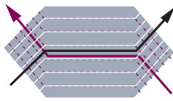
NEW (COUNTER-FLOW ELEMENT)
